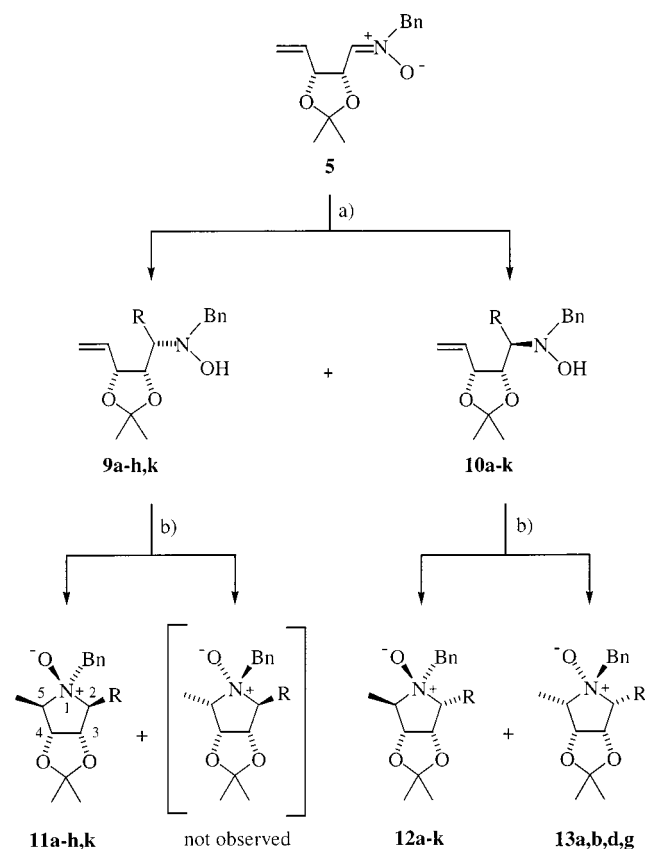
Scheme 4. Cope–House cyclization of the unsaturated hydroxylamines 9a–h,k and 10a–k generated by Grignard addition to the nitron 5: (a) RMgBr or RLi; (b) CHCl 3 ; cf. Table 1
