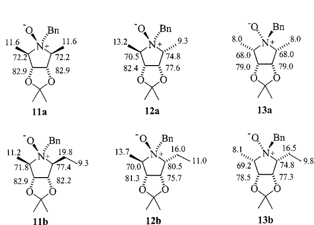
Figure 2. Comparison of ^{13}\text{C} NMR chemical shifts of 2-methyl- and 2-ethyl-substituted pyrrolidine N -oxides 11a–13a and 11b–13b
