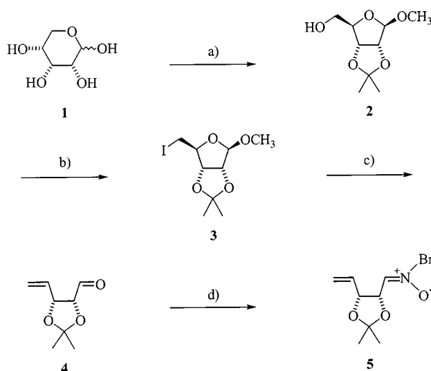
Scheme 2. Synthesis of the N -benzyl nitronone 5 from D-ribose ( 1 ): (a) 1. Me 2 C(OMe) 2 , MeOH, HCl, acetone, room temp., 21 h; 2. pyridine; 67%. – (b) PPh 3 , imidazole, I 2 , toluene, 70 °C, 2 h; 87%. – (c) n BuLi, THF, –80 °C, 2 h; quant. – (d) BnNHOH, MgSO 4 , CH 2 Cl 2 , room temp., 19 h; 69%
