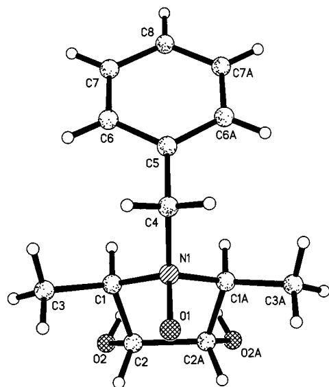
Figure 3. X-ray structure of the pyrrolidine N -oxide 16a
