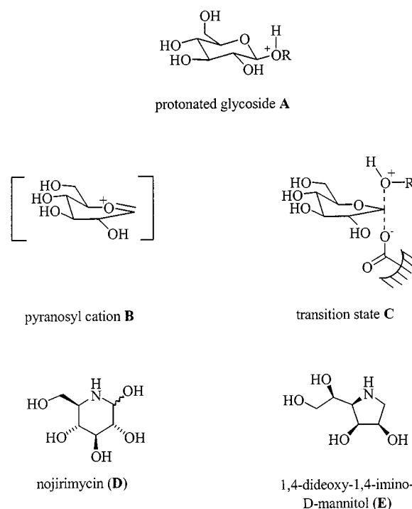
Figure 1. Intermediates and transition states proposed for enzymatic cleavage of glycosides. Iminoglycitols as examples of glycosidase inhibitors
