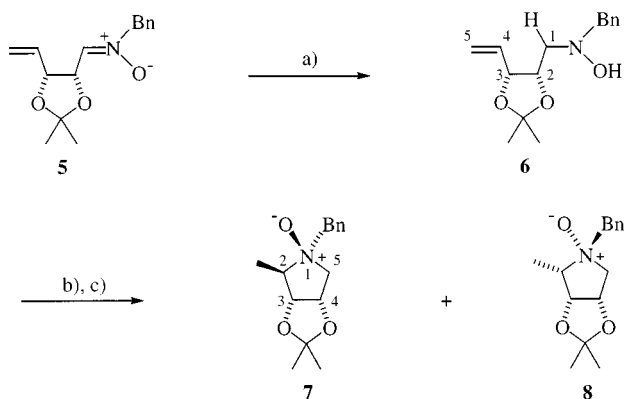
Scheme 3. Synthesis of the parent pyrrolidine N -oxides 7 and 8 by reduction of the nitron 5 : (a) \text{NaBH}_4 , EtOH, 0 °C, 4 h; (b) \text{CHCl}_3 , room temp., 16 h, 93%, 7/8 = 92:8; (c) crystallization; 7 : 66%
