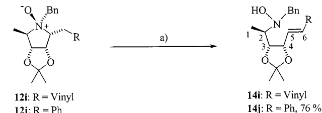
Scheme 5. Cope elimination of pyrrolidine N -oxides 12i and 12j: (a) Me 2 SO, 80 °C, 15–30 min
