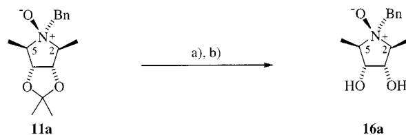
Scheme 7. O -deprotection of the pyrrolidine N -oxide 11a : (a) conc. HCl, MeOH, H 2 O (1:8:8), 1 d, room temp.; (b) Dowex 50WX8 (H + form); 84%
