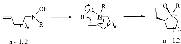
Scheme 1. Cope–House cyclization of unsaturated hydroxylamines
