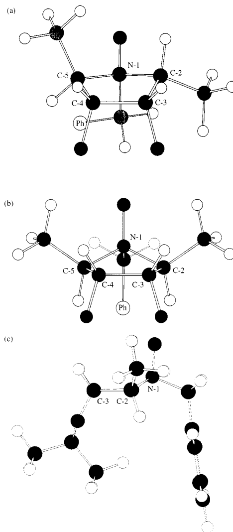
Figure 4. (a) and (b): Conformation of the pyrrolidine N -oxides 12a and 11a . The phenyl ring and the acetone group are omitted for clarity. (c) The side view of the pyrrolidine N -oxide 11a illustrates the symmetry of this conformer
