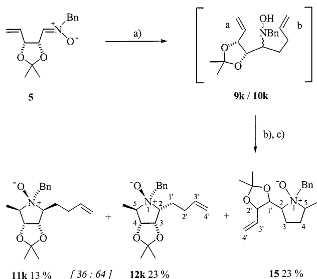
Scheme 6. Cope–House cyclization of the unsaturated hydroxylamines 9k/10k derived from nucleophilic addition of 3-butenylmagnesium bromide to the nitrone 5 : (a) 3-ButenylMgBr, Et 2 O, –20 °C, 3.5 h; (b) CHCl 3 , room temp., 5 d, isomer ratio 11k/12k/15 = 22:37:41; (c) MPLC; yields cf. above
